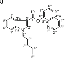
Quinolin-8-yl 1-pentyl-(1H-indole)-3-carboxylate (QUPIC, 1 ) C 23 H 22 N 2 O 2 : 358
