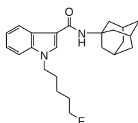
APICA N-(5-fluoropentyl) analog ( 5 ) C 24 H 31 FN 2 O: 382
