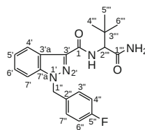
N-(1-Amino-3,3-dimethyl-1-oxobutan-2-yl)-1-(4-fluorobenzyl)-1H-indazole-3-carboxamide (ADB-FUBINACA, 3 ) C 21 H 23 FN 4 O 2 : 382
