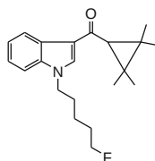
XLR11 (5FUR-144) C 21 H 28 FNO: 329
