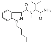
AB-PINACA
