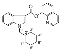
Quinolin-8-yl 1-(cyclohexylmethyl)-1H-indole-3-carboxylate (QUCHIC, 2 ) C 25 H 24 N 2 O 2 : 384
