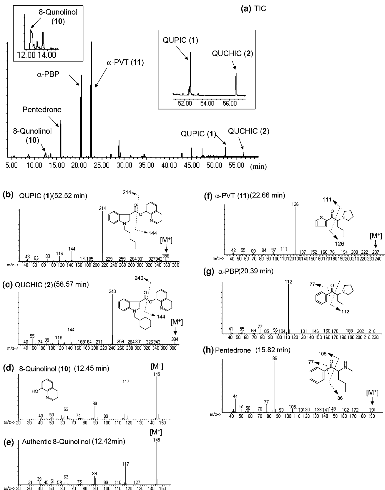
Fig. 3 Gas chromatography–mass spectrometry (GC–MS) analysis of product A. TIC (a) and electron ionization (EI) mass spectra of peaks 1 (b), 2 (c), 10 (d), 11 (f), α-PBP (g), pentedrone (h), and authentic 8-quinolol (e)
