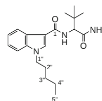
N-(1-Amino-3,3-dimethyl-1-oxobutan-2-yl)-1-pentyl-1H-indole-3-carboxamide (ADBICA, 4 ) C 20 H 29 N 3 O 2 : 343
