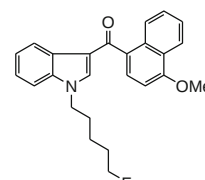
AM-2201 4-methoxynaphthyl analog (4-MeO-AM-2201, 9 ) C 25 H 24 FNO 2 : 389
