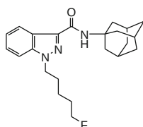
APINACA N-(5-fluoropentyl) analog ( 6 ) C 23 H 30 FN 3 O: 383
