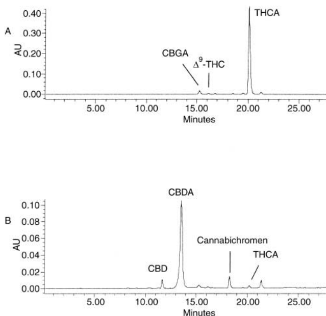
Figure 2. HPLC-chromatograms of the hexane extract of cannabis cultivars SIMM02 (A) and Kompolti (B). Main cannabinoid peaks are indicated.
