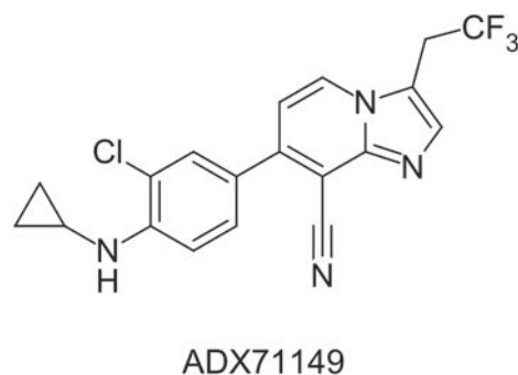
Fig. 5. Chemical structure of the selective mGlu 2 receptor positive allosteric modulator ADX71149.
