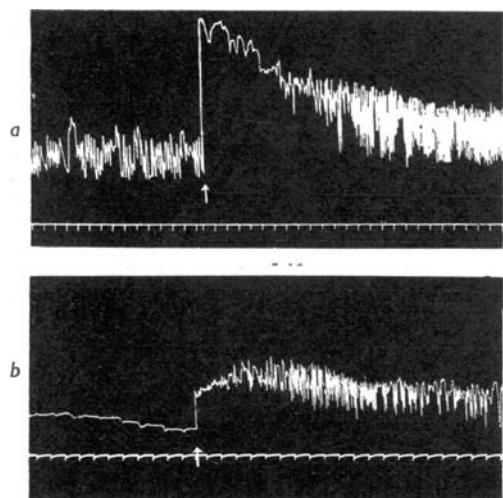
FIG. 2.—Liver fluke. Recordings as in Fig. 1. Effect of 5-hydroxytryptamine, 5 \times 10^{-4} M, (a) on intact parasite preparation, (b) on nerve-muscle preparation.
