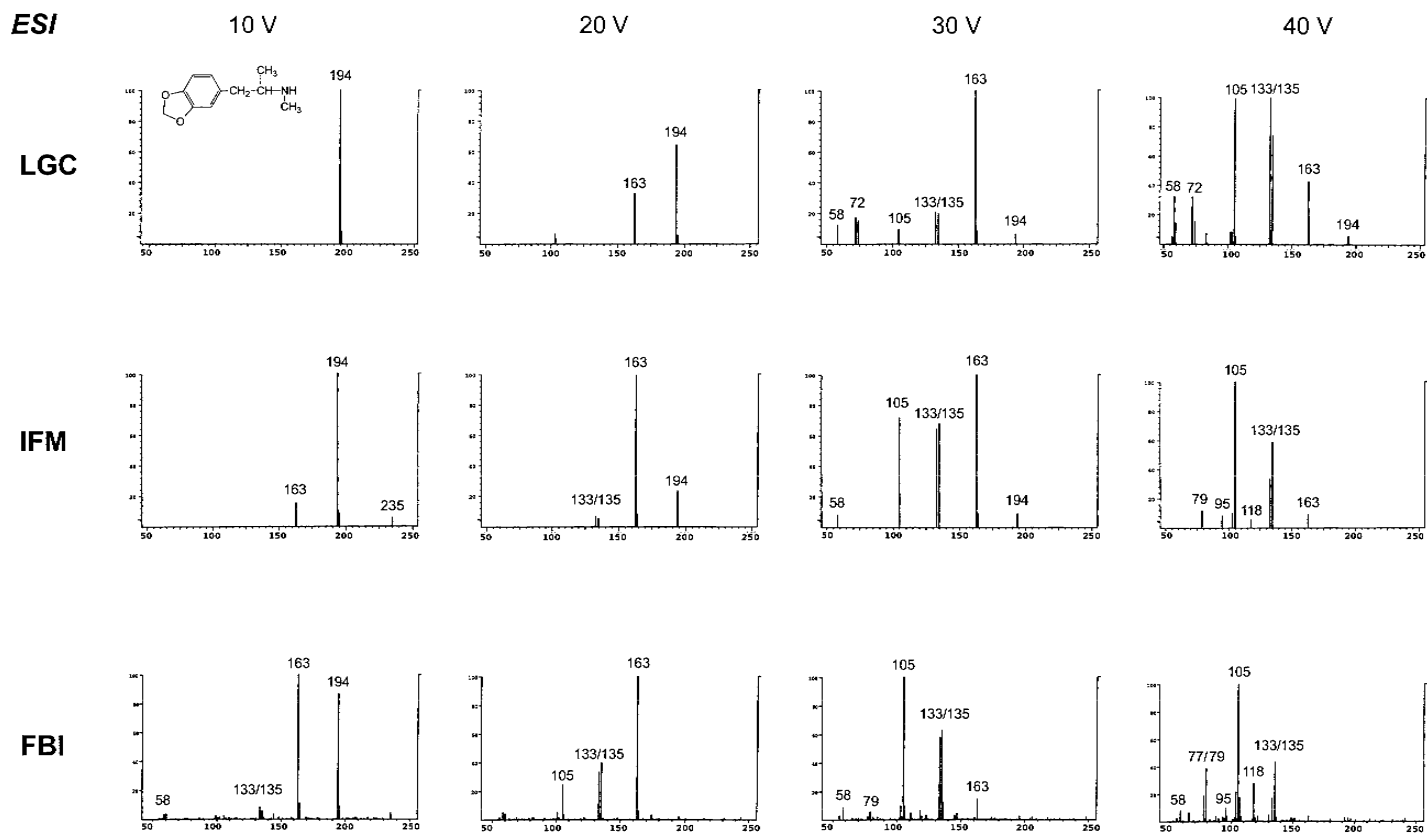
Fig. 2. Mass spectra of MDMA, taken in three participating laboratories in ESI mode at increasing octapole offset voltages (from 10 V to 40 V).
