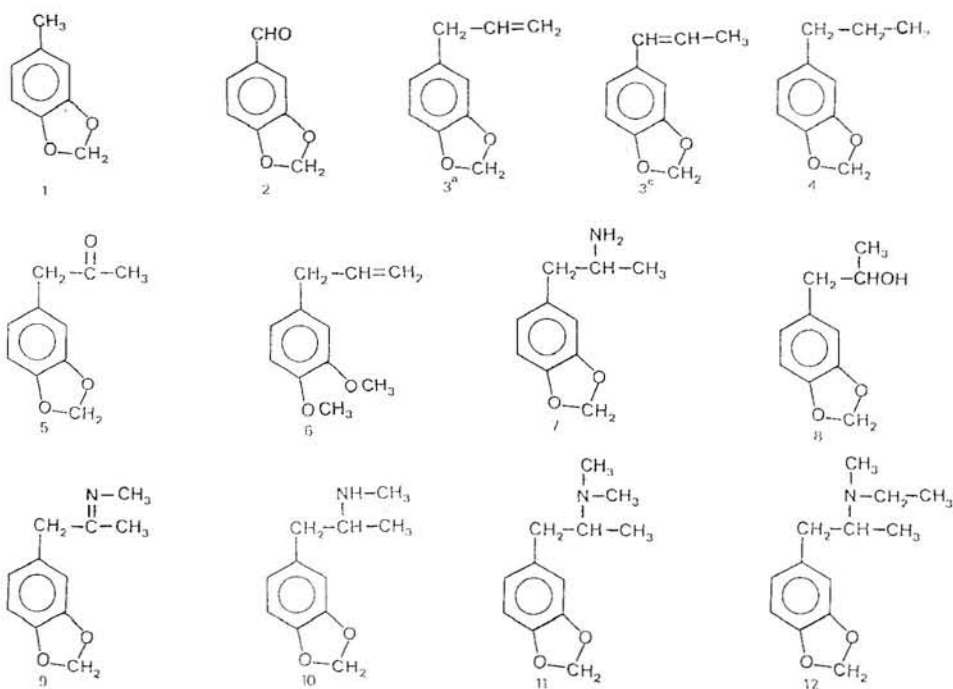
Fig. 3. Structural formulas of the compounds in Table 1.
