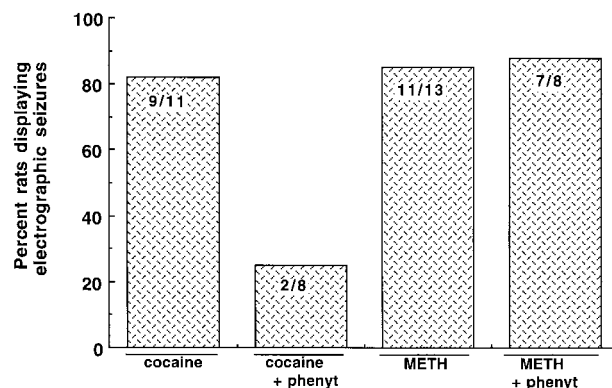
Fig. 3. Effect of phenytoin (Phenynt) on electrographic seizures induced by methamphetamine (METH; 40 mg/kg, i.p.) or cocaine (60 mg/kg, i.p.). Individual rats were pretreated with 10 mg/kg phenytoin 30 min prior to being challenged with either cocaine or methamphetamine. Results are plotted as a percent of animals displaying electrographic and behavioral seizures in each treatment group. The number of rats tested is shown in the columns (animals with clonic seizures/total rats tested).
