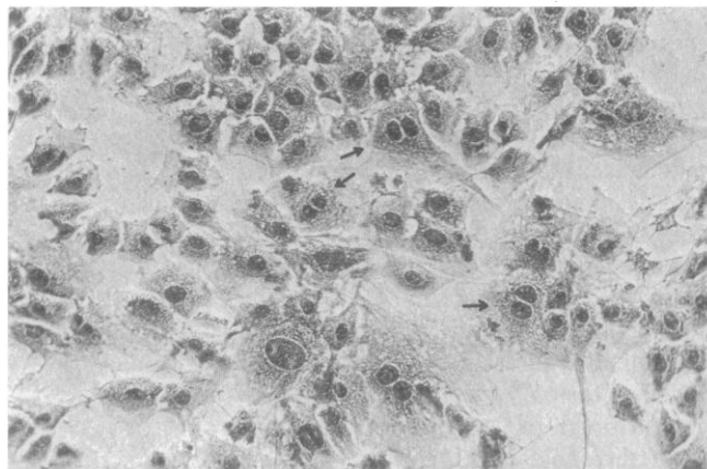
Fig. 1. Electric field-induced fusion of 3T3-C2 fibroblasts in monolayer culture. The cells were treated with five electric pulses of 1.6 kV/cm field strength and 100- \mu\text{sec} duration. A significant fraction of cells fused. Several binucleate cells are identified (see arrows for examples of fused cells). Fused cells were judged viable by the criteria discussed in the text.
