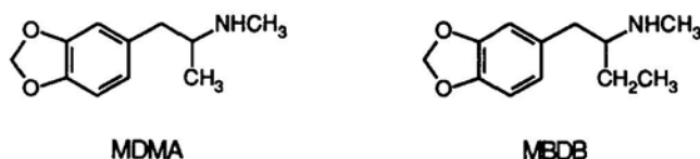
FIG. 1. The structures of MDMA and MBDB.
