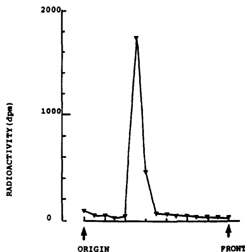
Fig. 5. The TLC analysis of radioactive materials in the brain of the mouse 3 hr after the intraperitoneal administration of [ 3 H]MDMA (15 mg/kg). Solvent system; CHCl 3 :MeOH:NH 4 OH = 9:1:0.1, R f value of MDMA (0.35).
