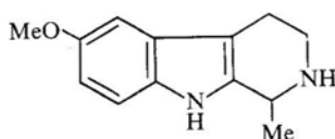
Fig. 1. Structure of \beta -carboline alkaloids.
