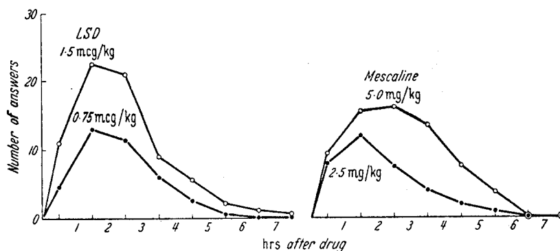
Fig. 2. Time course of subjective response after LSD and mescaline
