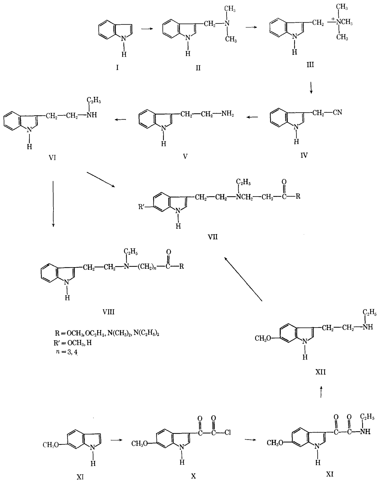
Scheme I
