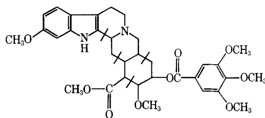
reserpine I
