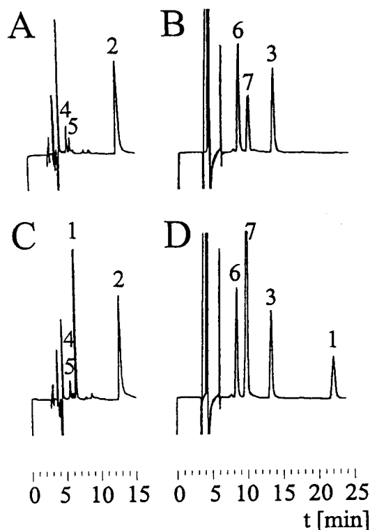
Fig. 2. HPLC chromatograms obtained from real plasma samples of volunteer 6 after 0 min (A, B) and 70 min (C, D) after p.o. administration of 0.2 mg/kg psilocybin. (A, C) LLE method; (B, D) on-line SPE method. 1=Psilocin; 2=5-hydroxyindole (I.S., LLE), 3=bufotenine (I.S., on-line SPE, 4, 5, 6, 7=biomolecules. Retention times in (C): 1=6.71 min, 2=13.62 min, 4=6.00 min, 5=6.18 min. Retention times in (D): 1=23.07 min, 3=13.86, 6=8.73, 7=10.13 min.
