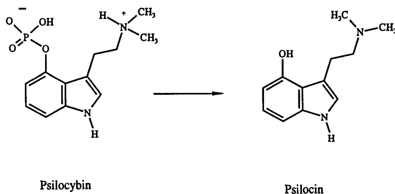
Fig. 1. Metabolism of psilocybin in the gut.
