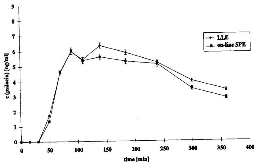
Fig. 3. Plasma concentration curves of psilocin (ng/ml) of volunteer 6 after p.o. administration of 10 mg psilocybin, comparison LLE with on-line SPE. Error bars: method standard deviation.
