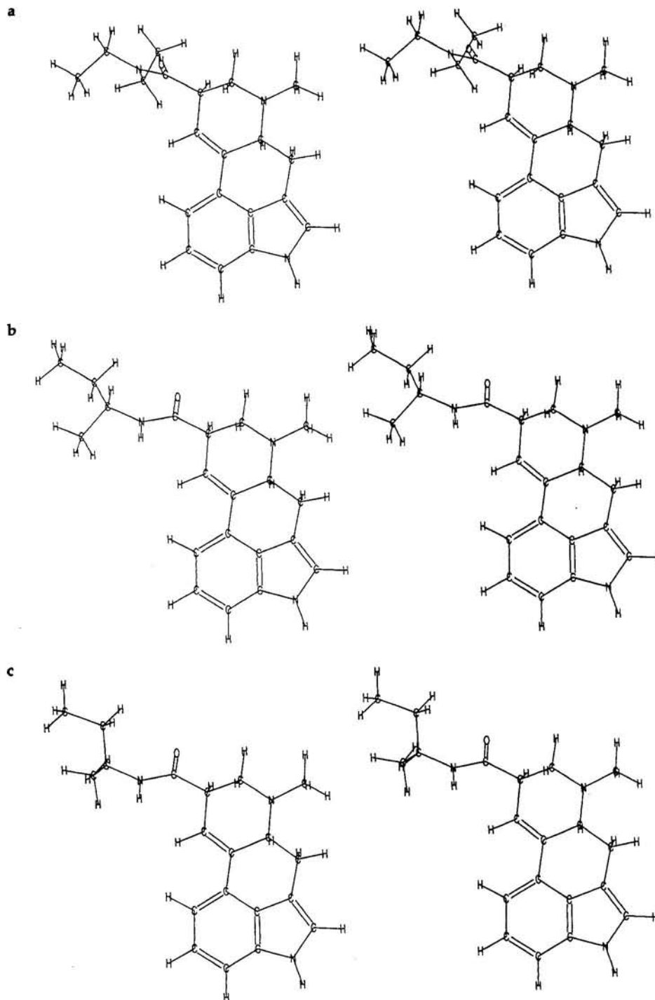
Figure 5. Stereoviews of fully minimized structures: (a) LSD (1), (b) ( R )-2-butyllysergamide (2), and (c) ( S )-2-butyllysergamide (3) as the free bases in the flap-up conformation.
