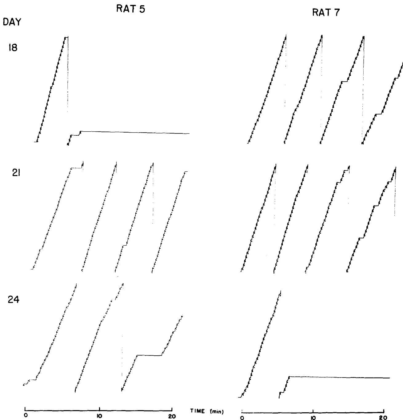
FIG. 4. Cumulative records showing the effects of daily precession or postsession treatment with LSD (100 \mu\text{g/kg} ). The records on the left (Rat 5) were obtained from an animal treated with LSD (100 \mu\text{g/kg} ) immediately before the operant session on Days 18–24. The records on the right were obtained from another animal (Rat 7) that was treated with LSD (100 \mu\text{g/kg} ) 30 minutes after the session on Days 18–23, and immediately before the session on Day 24. Rat 7 did not display tolerance to the disruptive effects of LSD on Day 24 when drug treatment was prior to the session. Rat 5 did however, develop a tolerance to the disruptive effects of LSD after 3 consecutive daily precession treatments.
