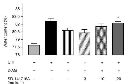
Figure 6 The protective effect of 2-AG is mediated by the CB 1 cannabinoid receptor. SR-141716A is a specific antagonist of the CB 1 brain receptor. Mice were subjected to CHI and 1 h later were injected with 2-AG (1 mg kg -1 ) and the antagonist (at 3, 10 or 20 mg kg -1 ). After 24 h they were killed and oedema was assessed. At its highest dose (20 mg kg -1 ), the antagonist significantly abolished the protective effect of 2-AG, suggesting that the latter affords its protection through its action at the CB 1 receptor. Asterisk, P < 0.05 versus 2-AG alone. Data are mean ± s.e.m.
