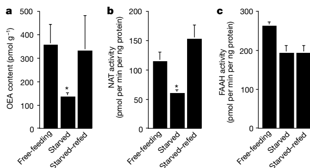
Figure 5 Feeding regulates OEA biosynthesis in small intestine. Effects of free feeding, starvation and starvation–refeeding on OEA levels ( a ), NAT activity levels ( b ) and FAAH activity levels ( c ). Asterisk, P < 0.05 ; n = 3 –5 per group.
