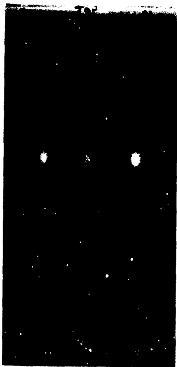
Fig. 5. TLC plate showing suspect LSD fraction viewed under UV light.
