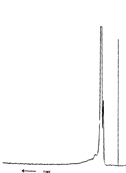
Fig. 2. HPLC trace of a control urine extract.
