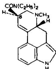
Fig. 1. Structural formula of LSD (iso-LSD has the opposite configuration at C-8).
