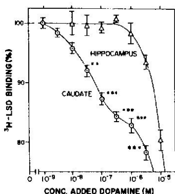
FIG. 4. Competition by dopamine for [ ^3\text{H} ]LSD binding in caudate and hippocampus
