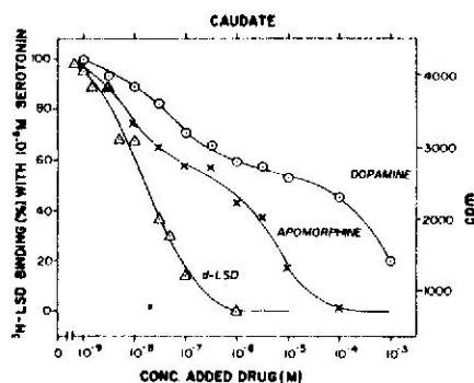
FIG. 5. Competition by dopamine, apomorphine, and d-LSD for [ ^3\text{H} ]LSD binding in the presence of 1 \mu\text{M} serotonin in membranes of calf caudate
