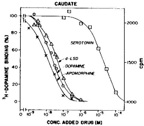
FIG. 1. Competition by dopamine, apomorphine, d -LSD, and serotonin for specific [ 3 H]dopamine binding in membranes of calf caudate
