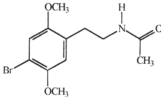
Figure 4 Acetylated 2C-B
