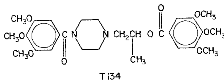
FIG. 2. Chemical structure of T-134.
