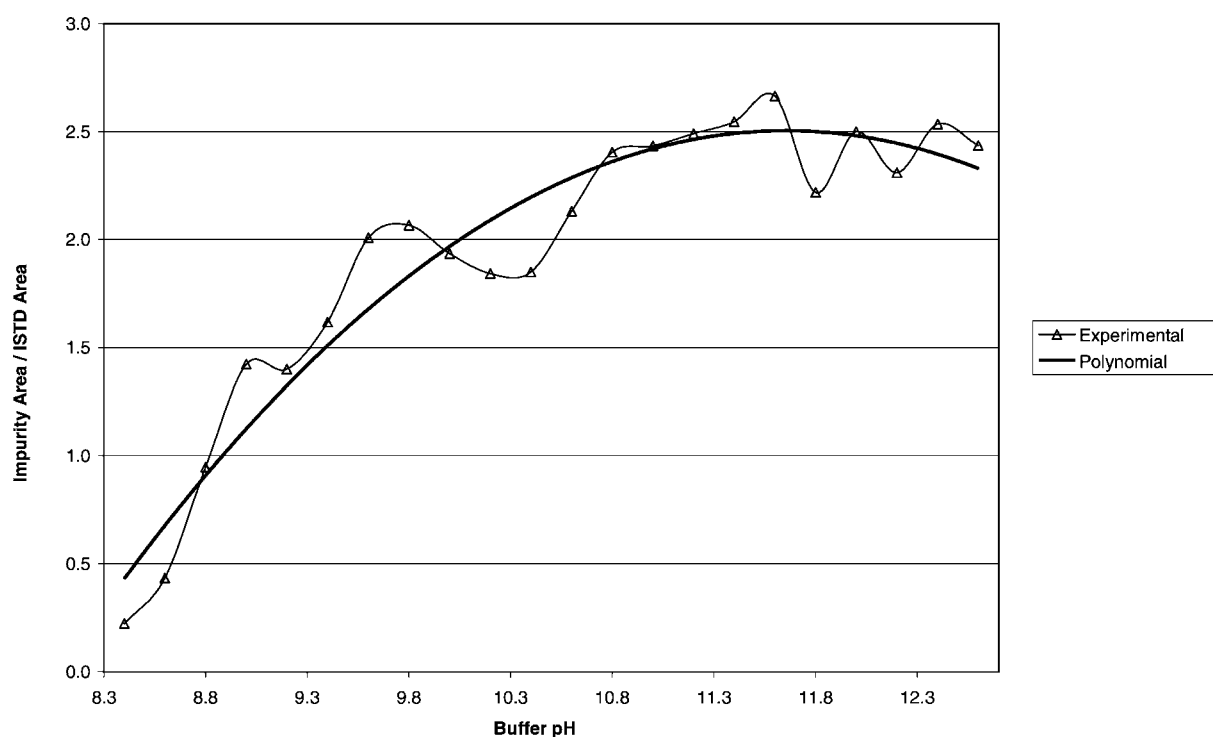
Fig. 3. Influence of pH on impurity 3.
