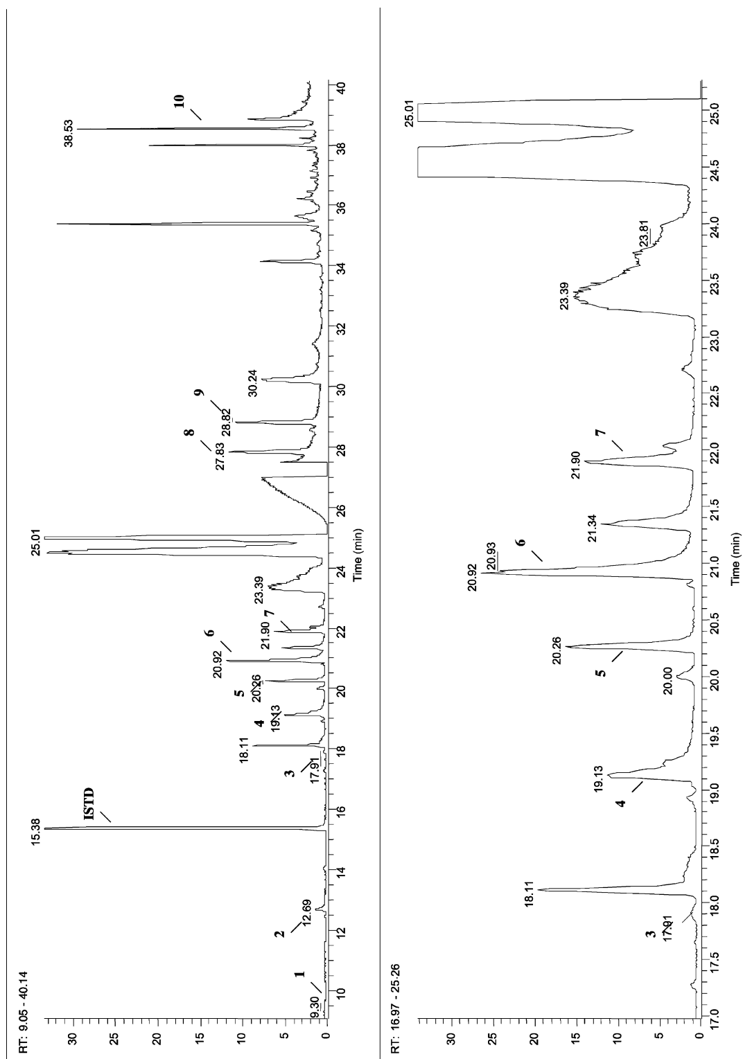
Fig. 1. Ei/full scan impurity profile of sample RefA.
