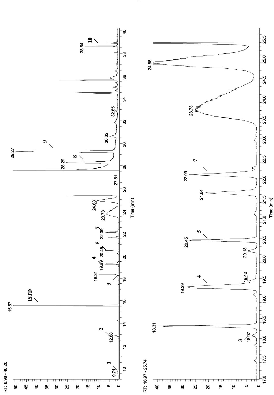
Fig. 2. ESI/Full scan impurity profile of sample RefB.
