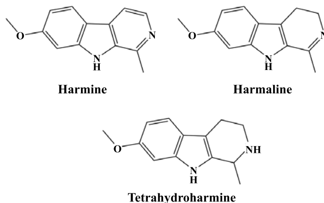
Fig. (2). Structures of harmine, harmaline and tetrahydroharmine.
