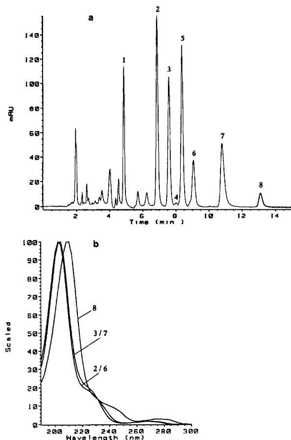
Fig. 1. (a) Chromatogram and (b) on-line UV spectra (DAD) of an extract of L. williamsii recorded at 205 nm. Peaks: 1 = anhalamine; 2 = mescaline; 3 = anhalonidine; 4 = isopellotine; 5 = methoxamine; 6 = N-methylmescaline; 7 = pellotine; 8 = anhalonine. Chromatographic conditions as described in Experimental.
