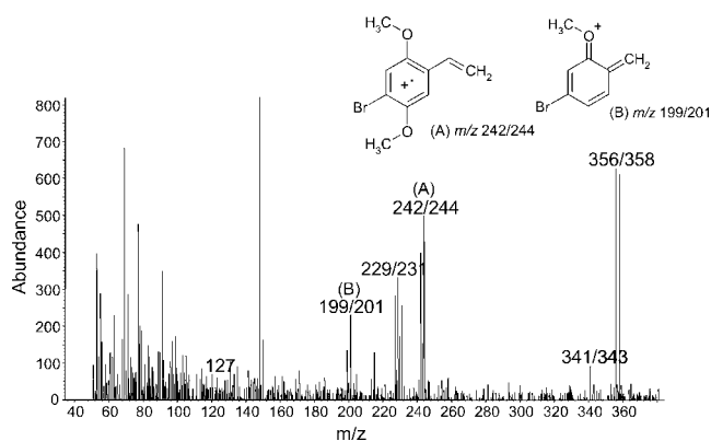
Fig. 3. Mass spectrum of the O -TFA derivative of the peak corresponding to the 2-(4-bromo-2,5-dimethoxyphenyl)-ethanol (BDMPE) metabolite observed in the chromatograms obtained with the mice urine samples extracted at basic pH. (A) Characteristic fragment at m/z 242/244; (B) characteristic fragment at m/z 199/201.
