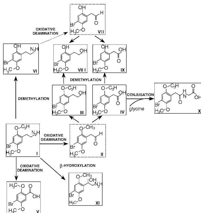
Fig. 7. Metabolic pathways found for 2C-B in mice after 24 h of acute drug administration. (I) 2C-B; (II) 4-bromo-2,5-dimethoxyphenylacetaldehyde; (III) BDMPE; (IV) BDMPAA; (V) BDMBA; (VI) B-2-HMPEA; (VII) 4-bromo-2-hydroxy-5-methoxyphenethylacetaldehyde; (VIII) B-2-HMPE; (IX) B-2-HMPAA; (X) BDMPA; and (XI) \beta -OH-2C-B. Structures outlined with full-line rectangles correspond to metabolites identified in the present study; structures outlined with discontinuous-line rectangles correspond to possible intermediate metabolites not identified in the present study.
