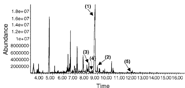
Fig. 4. Typical chromatogram obtained with the mice urine samples extracted at acidic pH. Peak identification 1, O -TMS derivative of 4-bromo-2,5-dimethoxyphenylacetic acid; 2, O -TMS derivative of 4-bromo-2-hydroxy-5-methoxyphenylacetic acid; 3, O -TMS derivative of 4-bromo-2,5-dimethoxybenzoic acid; 4, O -TMS derivative of 2-(4-bromo-2-hydroxy-5-methoxyphenyl)-ethanol; and 5, O -TMS derivative of 4-bromo-2,5-dimethoxyphenaceturic acid.
