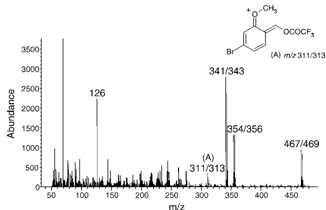
Fig. 2. Mass spectrum of the N,O -TFA derivative of the peak corresponding to the two \beta -hydroxylated 2C-B diastereomers ( \beta -OH-2C-B) observed in the chromatograms obtained with the mice urine samples extracted at basic pH. (A) Characteristic fragment at m/z 311/313.
