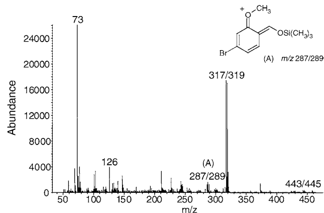
Fig. 1. Mass spectrum of the N -TFA- O -TMS derivative of the two peaks corresponding to the two \beta -hydroxylated 2C-B diastereomers ( \beta -OH-2C-B) observed in the chromatograms obtained with the mice urine samples extracted at basic pH. (A) Characteristic fragment at m/z 287/289.
