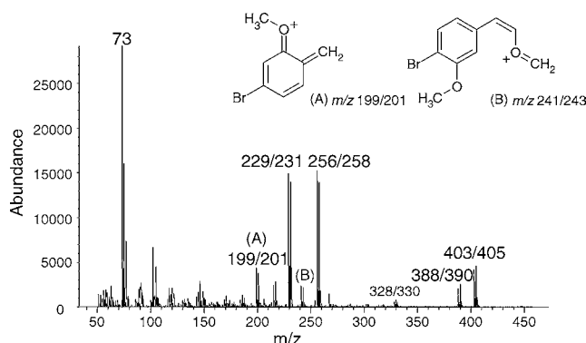
Fig. 5. Mass spectrum of the O -TMS derivative of the peak corresponding to the 4-bromo-2,5-dimethoxyphenacetic acid (BDMPA) metabolite observed in the chromatograms obtained with the mice urine samples extracted at acidic pH. (A) Characteristic fragment at m/z 199/201; (B) characteristic fragment at m/z 241/243.
