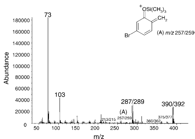
Fig. 6. Mass spectrum of the O -TMS derivative of the peak corresponding to the 2-(4-bromo-2-hydroxy-5-methoxyphenyl)-ethanol (B-2-HMPE) metabolite observed in the chromatograms obtained with the mice urine samples extracted at acidic pH. (A) Characteristic fragment at m/z 257/259.
