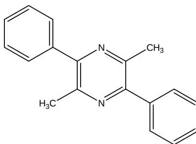
3,6 - dimethyl - 2,5 - diphenylpyrazine
