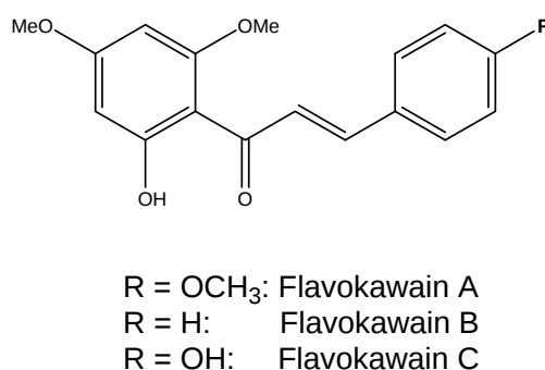
Figure 6. Chemical structures of flavokawains (FK) A, B, and C.
