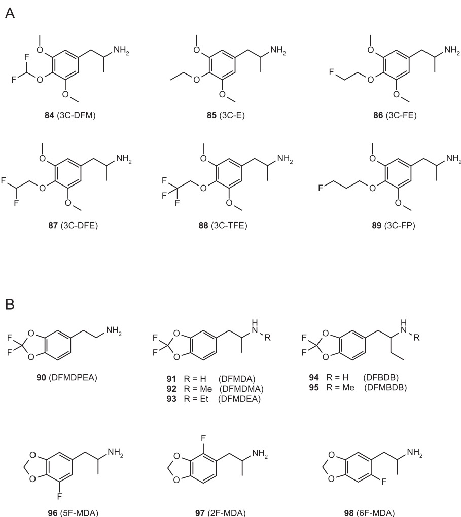
Figure 6. (A) 3,4,5-trisubstituted \alpha -methylated phenethylamines. (B) Fluorinated 3,4-methylenedioxyphenethylamines.
