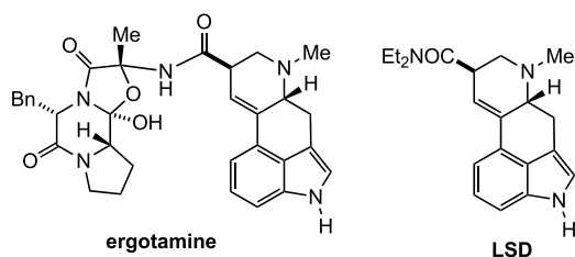
Figure 1. Structures of two representative ergot alkaloids.
