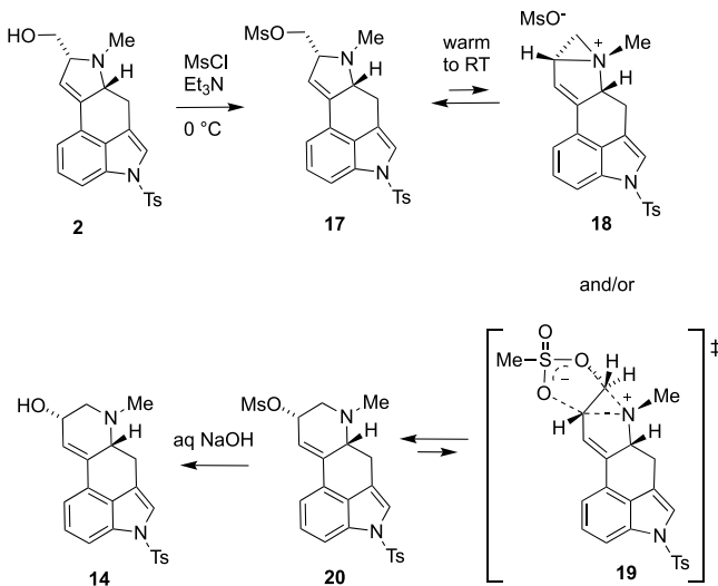
Scheme 4. Proposed Ring-Expansion Mechanism
