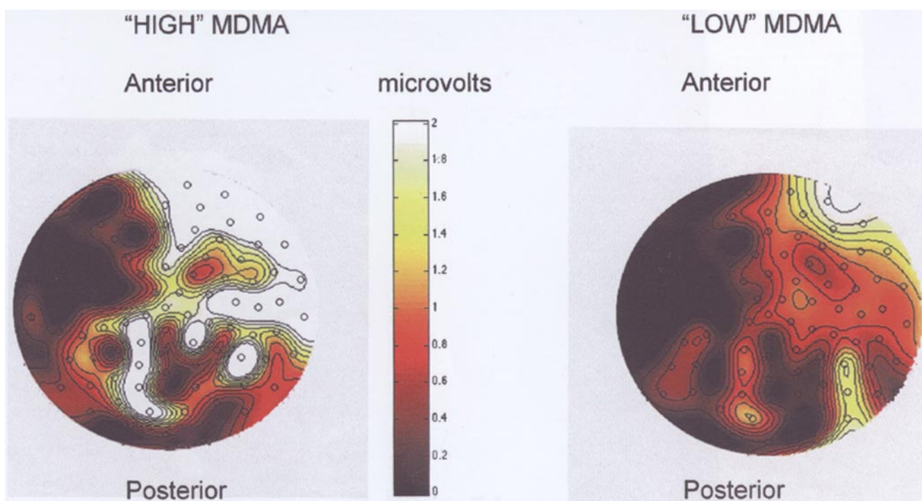
Fig. 2 Topography of mean alpha (9 Hz) power. Left , “high” MDMA users; right , “low” MDMA users (scale in \mu\text{V} ; n = 11 and 12, respectively). Front of the head is at the top in each figure
