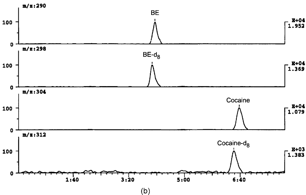
Fig. 1. Comparison of retention times of benzoylecgonine (BE) and cocaine on Superspher RP18 (a) and Discovery Amide C16 (b) columns. The same serum extract was examined, spiked with drugs to the concentration of 20 \mu\text{g/l} each.
