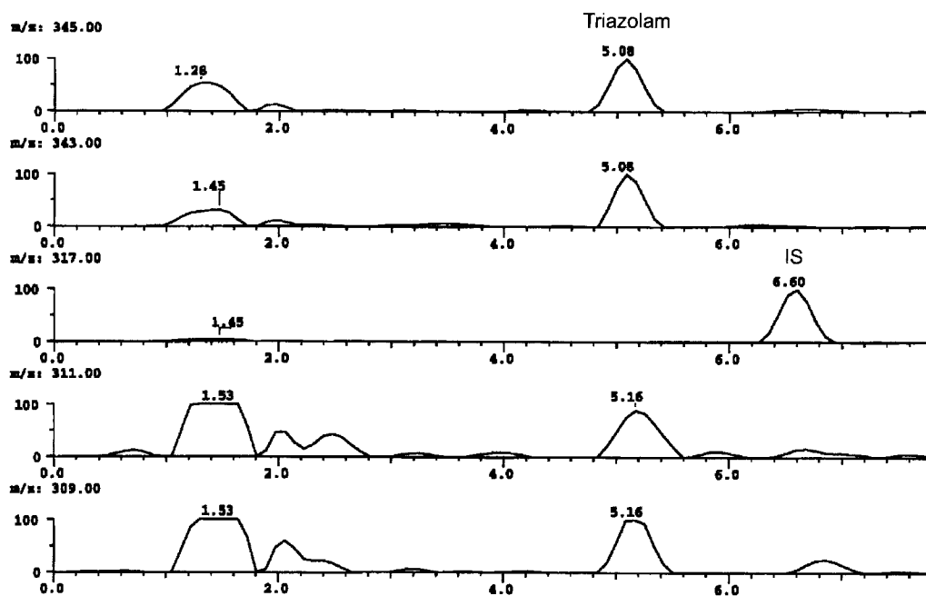
Fig. 8. Chromatogram of serum extract containing 8 \mu\text{g/l} of triazolam. Flunitrazepam-d3 was used as internal standard.
