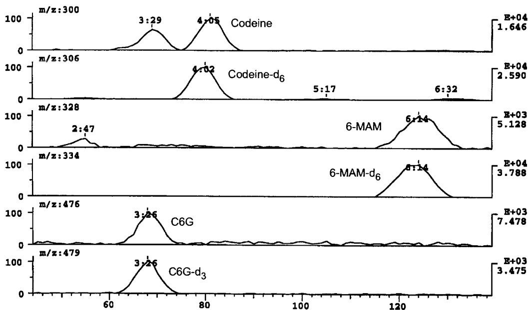
Fig. 3. Chromatogram of blood extract containing C6G 1533 \mu\text{g/l} , codeine 21 \mu\text{g/l} and 6-MAM 13 \mu\text{g/l} .
