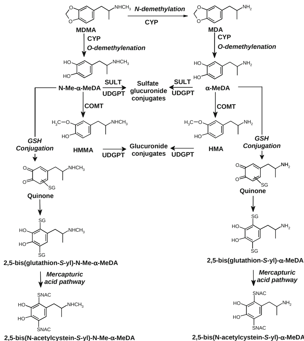
Fig. 5 Major pathways of MDMA metabolism. The parent compound is N -demethylated to form MDA and O -demethylated to form N -Me- \alpha -MeDA, which is further O -methylated to HMMA. In rats, N -demethylation to MDA is one of the main metabolic pathways, whereas in humans, O -demethylation to N -Me- \alpha -MeDA predominates. Isoenzymes of the cytochrome P450 (CYP) are involved in the N -demethylation and O -demethylation metabolic reactions. MDA is O -demethylated to form \alpha -MeDA. Both N -Me- \alpha -MeDA and \alpha -MeDA can undergo O -methylation to HMMA and HMA, respectively, a reaction regulated by catechol- O -methyltransferase (COMT). N -Me-
