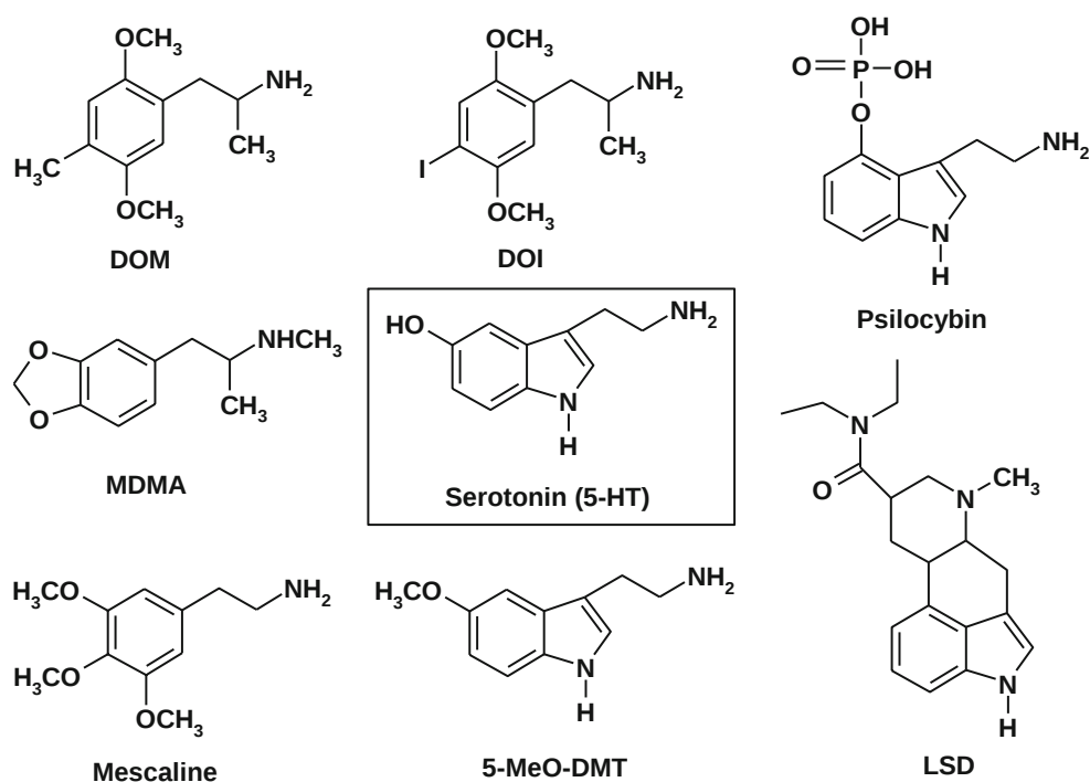
Fig. 3 Chemical structures of hallucinogenic compounds. These structures are closely related to the endogenous neurotransmitter 5-HT. DOI 1-(2,5-dimethoxy-4-iodophenyl)-2-aminopropane, DOM 1-(2,5-dimethoxy-4-methylphenyl)-2-aminopropane, 5-MeO-DMT 5-methoxy-N,N-dimethyltryptamine, LSD D-lysergic acid diethylamide
