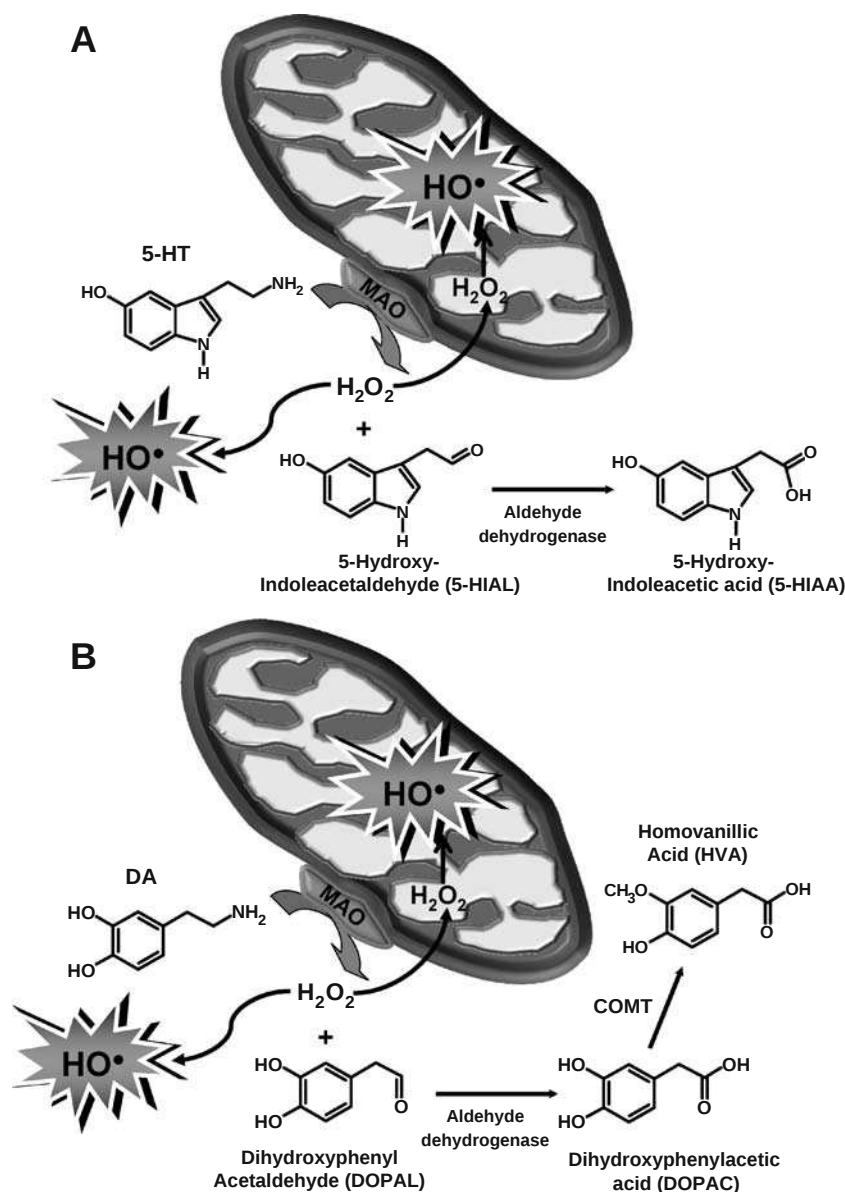
Fig. 7 Monoamine oxidase (MAO) located in the outer membrane of the mitochondria of neurons mediates the metabolism of serotonin (5-HT) in a and of dopamine (DA) in b . MAO-mediated metabolism of DA and 5-HT leads to the generation of the reactive aldehyde intermediates 3,4-dihydroxyphenylacetaldehyde (DOPAL) and 5-hydroxyindole-3-acetaldehyde (5-HIAL), respectively, before their conversion into the more stable metabolites 3,4-dihydroxyphenylacetic acid (DOPAC) and hydroxyindole-3-acetic acid (5-HIAA) by
