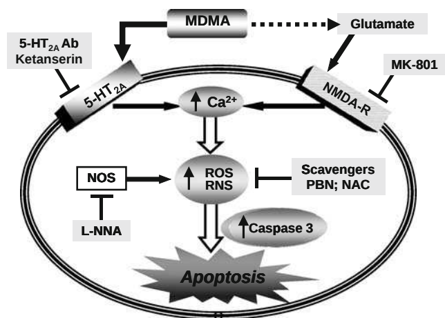
Fig. 8 Postulated mechanism of MDMA-induced neurodegeneration in cortical neurons. Direct activation of 5-HT 2A -receptors by MDMA may induce neuronal death, which can be attenuated by the competitive antagonists ketanserin or R-96544 and completely blocked by the antibody (5-HT 2A Ab) for that receptor. Moreover, MDMA might elicit GLU release either directly or indirectly via 5-HT 2A -receptor-mediated cell death, which will act on NMDA-receptors (NMDA-R), an effect that can be antagonized by MK-801. Both 5-HT 2A and NMDA receptors activation will lead to an increase in iCa^{2+} levels. This increase will activate NOS activity, leading to the overproduction of NO and subsequently to the formation of damaging peroxynitrite. Both nNOS and iNOS activity can be inhibited by selective and non-selective antagonists, like L-NNA. Under this scenario of oxidative stress, ROS/RNS can be scavenged by the antioxidants, NAC and PBN. Ultimately, neurons will undergo apoptotic death accompanied by caspase 3 activation
