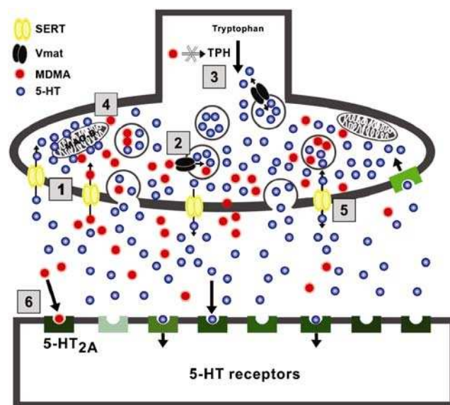
Fig. 2 MDMA pharmacological mechanism of action at the neuronal serotonergic terminal and synapse. 1 MDMA, like serotonin (5-HT), is a substrate of the serotonin transporter (5-HTT) and uses the transporter to enter inside the neuronal terminal, although at high concentration, it may also enter by diffusion. 2 Once inside, MDMA produces an acute and rapid enhancement in the release of 5-HT from the storage vesicles, possibly by entering the vesicles via the vesicular monoamine transporter (VMAT) and depletes vesicular neurotransmitter stores via a carrier-mediated exchange mechanism. 3 MDMA also inhibits tryptophan hydroxylase (TPH), the rate-limiting enzyme for 5-HT synthesis. 4 Monoamine oxidase B (MAO-B), located in the outer membrane of the mitochondria of serotonergic neurons, is the enzyme responsible for 5-HT degradation and its activity is partially inhibited by MDMA. 5 Due to the increase in the free cytoplasmic pool of 5-HT, MDMA promotes a rapid release of intracellular 5-HT to the neuronal synapse via reversal of the 5-HTT activity. 6 MDMA hallucinogenic properties depend on the agonist activity at the 5-HT 2A -receptor
