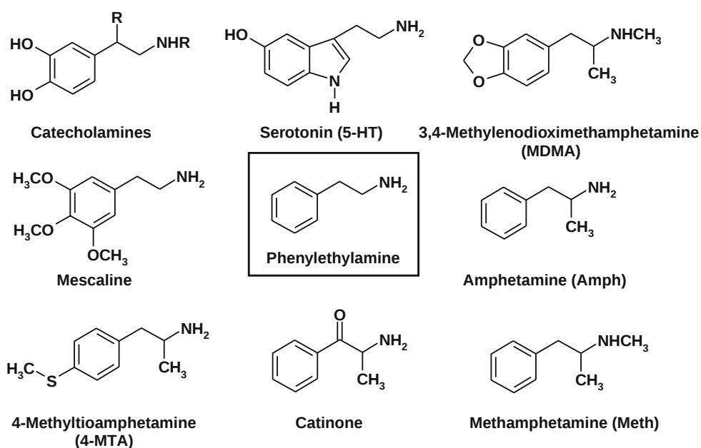
Fig. 1 Chemical structures of MDMA (“ecstasy”) and related amphetamines. Amphetamines are phenylethylamine derivatives chemically related to the monoamine neurotransmitters and to the naturally occurring hallucinogenic compounds, like mescaline and catinone. Mescaline is found in the peyote cactus that grows in North America. Catinone is present in the leaves of the Khat plant, native to the sub-Saharan, which is chewed in many Arabic countries to combat starvation and fatigue during the Ramadan period or even on a daily basis in social occasions
