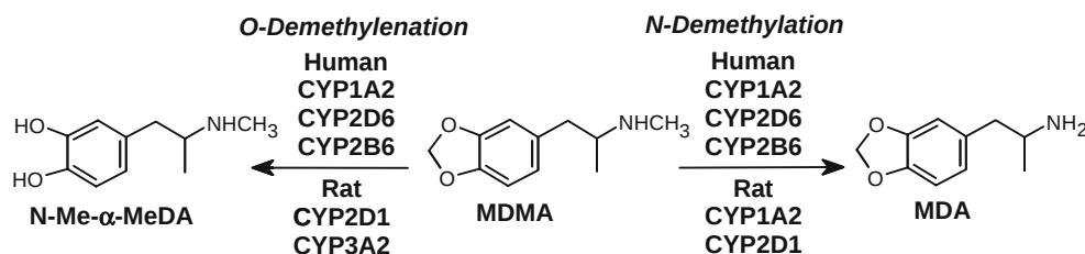
Fig. 6 Major CYP isoenzyme-dependent MDMA metabolic pathways in humans and rats. Data are taken from [69] and [55]
