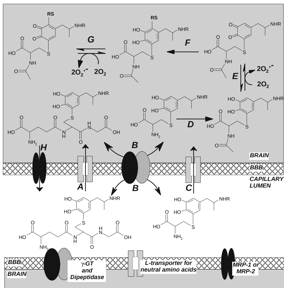
Fig. 10 Postulated model for the delivery of GSH-conjugated MDMA metabolites into the brain. a Both 5-(GSH)-N-Me- \alpha -MeDA (R=CH 3 ) and 5-(GSH)- \alpha -MeDA (R=H) can be transported into the brain by L-transporter for neutral amino acids located in the capillaries of the blood–brain barrier (BBB). b These conjugates can be metabolized by \gamma -GT and dipeptidase to their correspondent cysteine derivates either in the brain or even in the capillary lumen. c Cysteine conjugates formed in the capillary lumen can also be transported into the brain by the L-transporter for neutral amino acids. d By N-acetyltransferase action, cysteine conjugates can be further metabolized to their correspondent NAC conjugates. NAC conjugates appear
