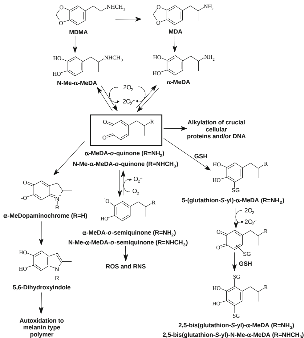
Fig. 9 Postulated mechanisms for production of MDMA toxic derivatives like ortho -quinones, semiquinones, and amino-chrome. The catechols are readily oxidized to their corresponding ortho -quinones in the presence of catalytic amounts of transition metal ions, which can enter redox cycle and generate semiquinone radicals, leading to the formation of ROS and RNS. Alternatively, ortho -quinones can undergo adduction with nucleophiles like GSH, proteins, or even DNA. On cyclization, ortho -quinones give rise to the formation of amino-chromes and related compounds, such as 5,6-dihydroxyindoles, which can undergo further oxidation and polymerization to form brown or black insoluble pigments of melanin type. Adapted from [76]
