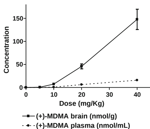
Fig. 4 (+)-MDMA concentration time-curves in the plasma and brain as a function of the (+)-MDMA dose given to Sprague–Dawley rats. MDMA concentrations rise in a nonlinear manner with the increase of MDMA dose. The expected brain concentrations of MDMA, assuming a linear trend of concentrations with increasing doses, would be much lower than the ones actually found. The rate of MDMA conversion to 3,4-methylenedioxymphetamine (MDA) by N -demethylation, the main metabolic pathway in rats, becomes saturated at higher dosage of MDMA. Data were taken and reworked from [50]
