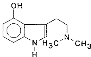
Figure 1. Molecular structures of psilocybin and psilocin.
