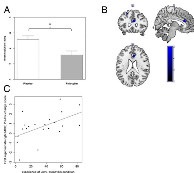
Fig. 1. (A) Social exclusion feelings were significantly reduced after Psi vs. Pla administration. Data are expressed as means + the SEM ( n = 21 subjects). Asterisks indicate significant differences between Psi and Pla conditions ( *P < 0.05 ). (B) fMRI activation data for Pla > Psi in the "not receiving ESE > receiving INCL" contrast. Blue shades represent significantly reduced activation in the Psi condition displayed at uncorrected P < 0.001 at peak aMCC voxel ( x = 6, y = 26, z = 22 ). (C) Positive association between the experience of unity assessed by the 5D-ASC questionnaire and right MCC activation in the "not receiving ESE > receiving INCL" contrast ( r = 0.53, P < 0.02, n = 21 ; first eigenvariate; Pla–Psi change score).
