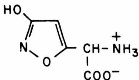
IBOTENIC ACID
