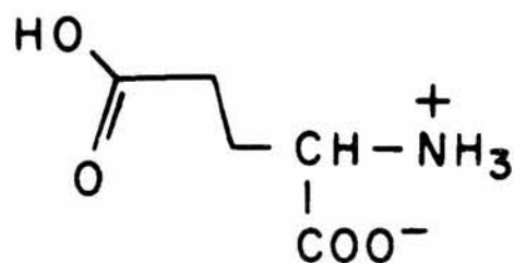
GLUTAMATE
