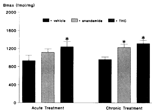
FIG. 1. Maximum binding capacity ( B_{\max} ) of cannabinoid receptors in the cerebellum of male rats acutely or chronically exposed to either anandamide or \Delta^9 -tetrahydrocannabinol (THC). Details in the text. Values are means \pm SEM of six to eight determinations per group. Data were analyzed by two-way ANOVA (* p < 0.05 vs. the corresponding control).
