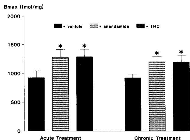
FIG. 2. Maximum binding capacity ( B_{\max} ) of cannabinoid receptors in the hippocampus of male rats acutely or chronically exposed to either anandamide or \Delta^9 -tetrahydrocannabinol (THC). Details in the text. Values are means \pm SEM of six to eight determinations per group. Data were analyzed by two-way ANOVA (* p < 0.05 vs. the corresponding control).
