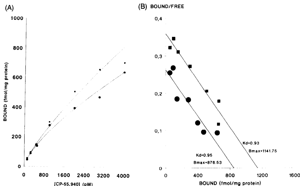
FIG. 6. Saturation curve (A) and Scatchard plot (B) of a representative [^3\text{H}]\text{CP-55,940} binding assay using membranes of the striatum of male rats chronically exposed to \Delta^9 -tetrahydrocannabinol (●) or vehicle (■). Details in the text.
