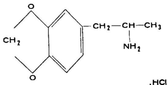
FIG. 1. Structural formula of SKF #5
