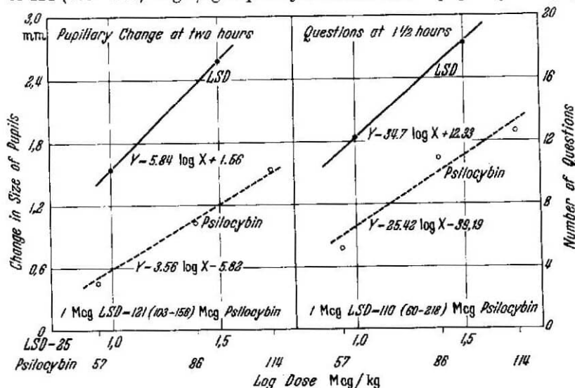
Fig. 1. Relationship of dose of LSD-25 and psilocybin to change in size of pupils and to number of positive responses on the questionnaire
