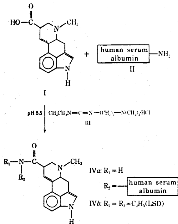
Scheme 1—Covalent coupling of lysergic acid (I) to human serum albumin (II) by a water-soluble carbodiimide reagent (III), producing antigen (IVa)
