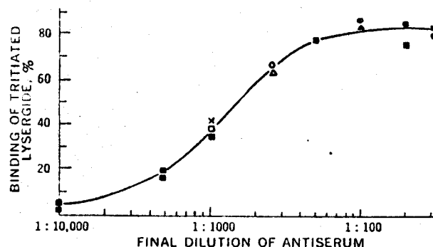
Figure 1—Binding of tritiated lysergide (1.0 ng./ml.) by antiserum to a lysergic acid-human serum albumin conjugate. Key: \bullet , \circ , \Delta , \square , \times , data as given in Table I and Fig. 2; and \blacksquare , additional experimental results.
