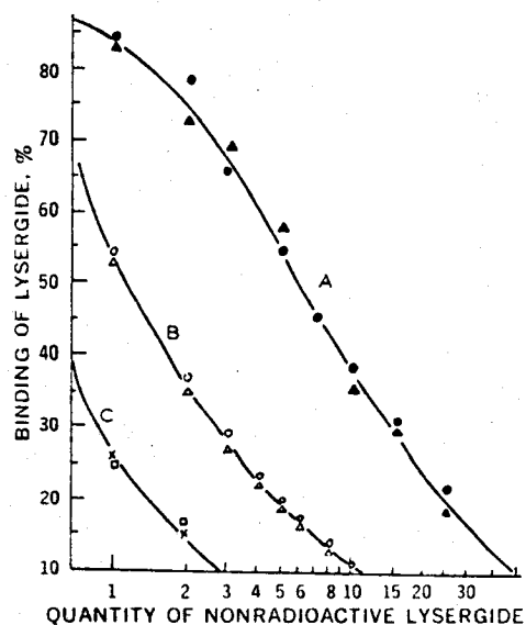
Figure 2—Typical standard radioimmunoassay curves for the determination of lysergide at three antiserum dilutions (A, 1:100; B, 1:400; and C, 1:1000). Key: \bullet , \circ , \Delta , and \times indicate duplicate assay results. The curves shown have not been mathematically fit.
