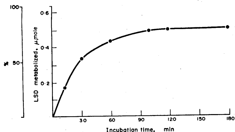
FIG. 1. Time course for the metabolism of LSD by rat liver 9000 g supernatant fraction. Incubation mixture contained 3 ml of 9000 g supernatant fraction, 0.63 \mu\text{mole} of LSD, 1 \mu\text{mole} of NADP, 100 \mu\text{moles} of nicotinamide, 100 \mu\text{moles} of \text{MgCl}_2 , 0.5 ml of 0.8 M phosphate buffer (pH 7.4), and water to make a final volume of 5 ml.
