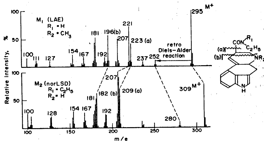
FIG. 2. Mass spectra of the metabolites M_1 (LAE) and M_2 (norLSD). Mass spectra were measured by a direct insertion probe technique: sample temperature, 150–200°; ion-chamber temperature, 100–200°; ionizing energy, 75 eV; ionizing current, 200 \mu A.
