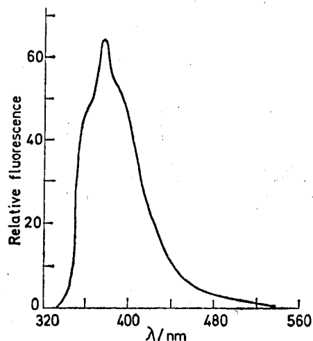
FIGURE 1 Corrected fluorescence spectrum of ergometrine in ethanol at 77 K ( \lambda_{\text{ex}} = 320 \text{ nm} )
