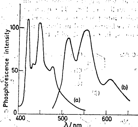
FIGURE 2 Phosphorescence spectra of (a) agroclavine and (b) ergometrinine in ethanol at 77 K (the spectrum of ergometrinine has been scaled up by a factor of 100)
