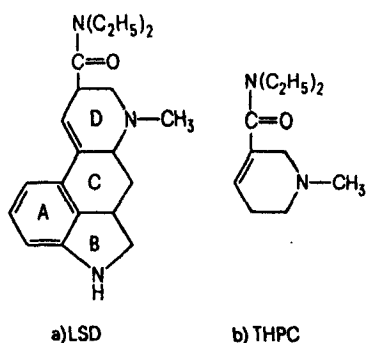
Fig. 1. Structural relationship between a) n -lysergic acid diethylamide and (LSD) b) 1-methyl-1, 2, 5, 6-tetrahydropyridine- N , N -diethylcarboxamide (THPC).
