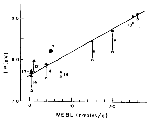
Figure 13. Plot of the first \pi ionization potential and the average of the first two \pi ionization potentials ( IP 's) of hallucinogens and related compounds vs. the minimum effective brain level (MEBL) to alter rat behavior in a conditioned avoidance response. (19 = LSD; 18 = 5-methoxydimethyltryptamine; 17 = 5-methoxytryptamine; 14 = dimethyltryptamine; 7 = mescaline; 6 = 3,4-dimethoxyphenethylamine; 5 = 4-methoxyphenethylamine; 10 = amphetamine; 1 = phenethylamine; 12 = tryptamine after MAO inhibition. Tryptamine derivatives: IP_1 = \Delta and IP_{av} = \bullet . Phenethylamine derivatives: IP_1 = O and IP_{av} = \bullet .) The line is for IP_{av} .
