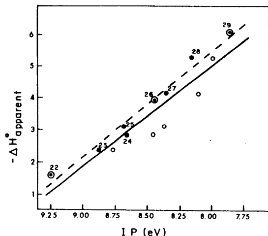
Figure 12. Plots of apparent enthalpies of formation of aromatic hydrocarbon-TCNE complexes vs. IP_1 (O) or IP_{av} = (IP_1 + IP_2)/2 (●) of the aromatic hydrocarbon: 22, benzene; 23, toluene; 24, o -xylene; 25, p -xylene; 26, mesitylene; 27, 1,2,4,5-tetramethylbenzene; 28, pentamethylbenzene; 29, hexamethylbenzene. Solid line is for IP_1 ; broken line is for IP_{av} .
