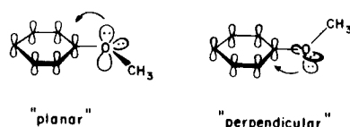
Figure 5. "Planar" and "perpendicular" conformations of anisole.
