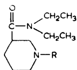
1-Substituted N,N-Diethylnipecotamides.
