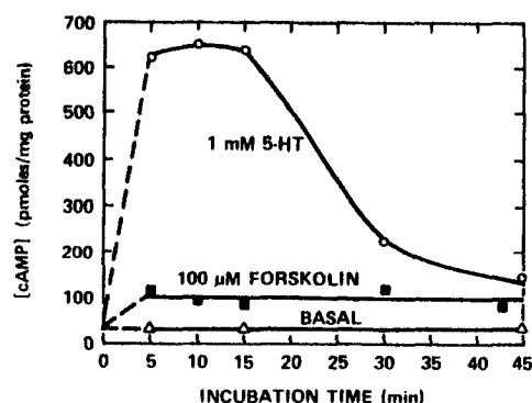
Fig. 7. Effect of forskolin on cAMP levels in intact flukes. Liver flukes were incubated at 37° in media containing no additions ( \Delta ), 100 \mu M forskolin ( \blacksquare ), or 1 mM 5-HT ( \circ ). At the indicated incubation times, the cAMP content from an aliquot of flukes was determined by radioimmunoassay as described in Methods and Materials. The results are mean values from duplicate samples of a single experiment.
