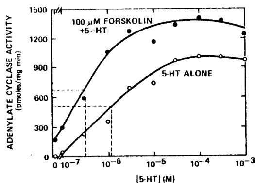
Fig. 3. Effect of forskolin on 5-HT activation of adenylylase. Fluke particles were assayed for adenylylase activity as described in Methods and Materials in the presence of the indicated concentrations of 5-HT and 100 \mu M GTP with no additions ( \circ ) or with 100 \mu M forskolin ( \bullet ). The values given are means from duplicate samples of a representative experiment.
