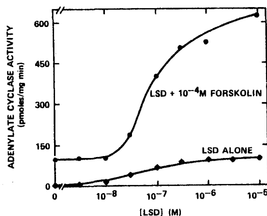
Fig. 4. Effect of forskolin on LSD activation of adenylylase. Fluke particles were assayed for adenylylase activity as described in Methods and Materials in the presence of the indicated concentrations of LSD plus 100 \mu M GTP with no additions ( \circ ) or with 100 \mu M forskolin ( \bullet ). The values given are means from duplicate samples of a representative experiment. In the same preparation, 100 \mu M 5-HT activated adenylylase to a level of 1040 pmoles/mg \cdot min and 100 \mu M 5-HT + 100 \mu M forskolin activated the enzyme to 1540 pmoles/mg \cdot min.
