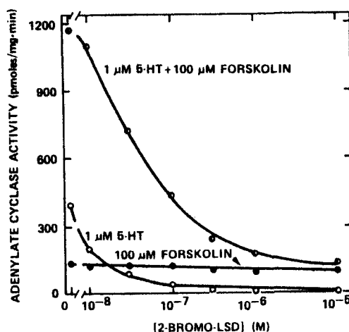
Fig. 5. Effect of 2-bromo-LSD on forskolin activation of adenylylase. Fluke particles were assayed for adenylylase activity as described in Methods and Materials in the presence of the indicated concentrations of 2-bromo-LSD with 1 \mu M 5-HT and 100 \mu M GTP ( \circ ), with 100 \mu M forskolin ( \bullet ), or with 1 \mu M 5-HT and 100 \mu M GTP plus 100 \mu M forskolin ( \bullet ). The values given are means from duplicate samples of a representative experiment. The basal adenylylase activity in this experiment was 6 pmoles/mg \cdot min.
