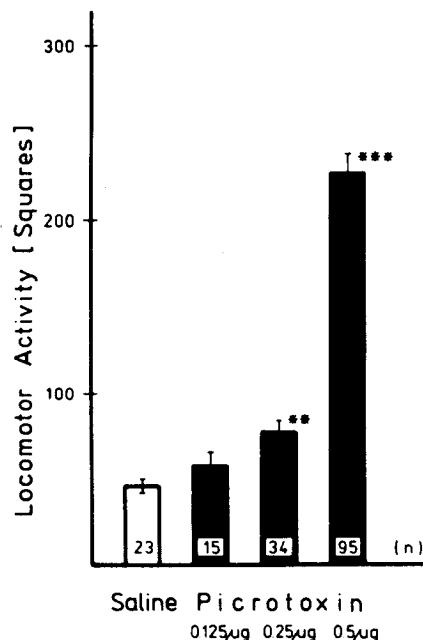
FIG. 1. Bilateral IA injection of PIC induces a dose-dependent increase of locomotor activity. Vertical bars represent the means \pm S.E.M. of (n) animals. ** p < 0.005 , *** p < 0.001 vs. saline (Mann-Whitney).
