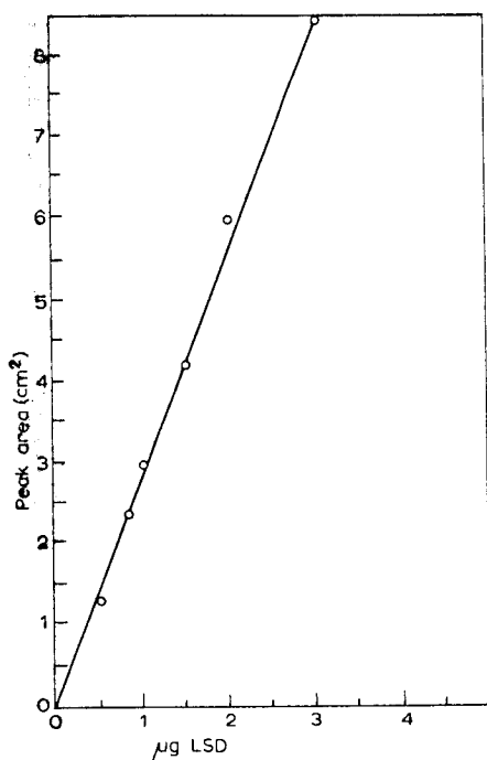
Fig. 2. A standard calibration curve of LSD.
