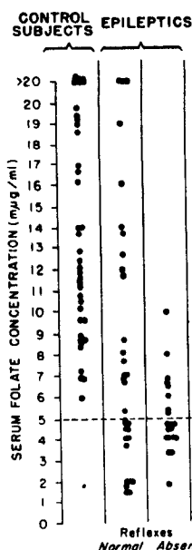
Serum-folate concentrations in control subjects and in epileptic patients.
