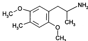
DOM (2,5-dimethoxy-4-methylamphetamine)
