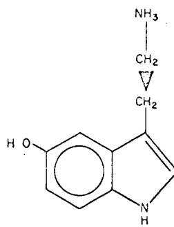
Fig. 3—Calculated charge densities ( \sigma + \pi ) for serotonin.
