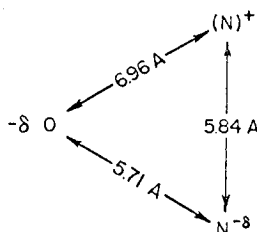
Fig. 5—Structural features proposed as being complementary to the serotonin receptor.
